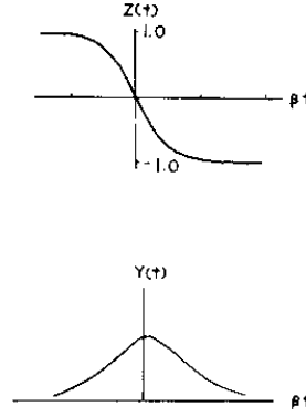
FIG. 1. The time dependence of the energy and of the amplitude of the dipole moment for spontaneous emission.
