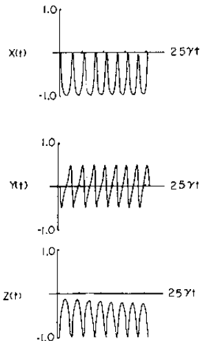
FIG. 8. Solutions of the secular equations for \alpha = \beta = 0 , and \lambda < \frac{1}{2}\gamma .
