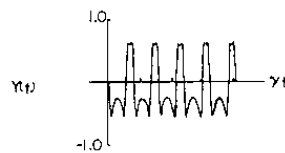
FIG. 11. Solutions of the general secular equations with a strong applied field, \alpha=0 , \beta=0.1\gamma , and \lambda > \frac{1}{2}\gamma .
