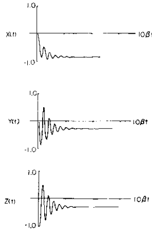
FIG. 6. Solutions of the secular equations for strong applied field off resonance, \gamma = 0 , \alpha = \beta , and \lambda = 3\beta .
