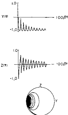
FIG. 5. Solutions of the secular equations for \alpha < 0.01\beta , \lambda \approx 1.01\beta , and \gamma = 0 .
