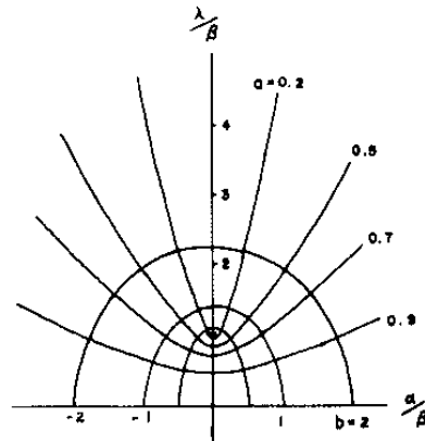
FIG. 3. The decay constants and oscillation frequencies for transients after sudden turn on of the driving field.
