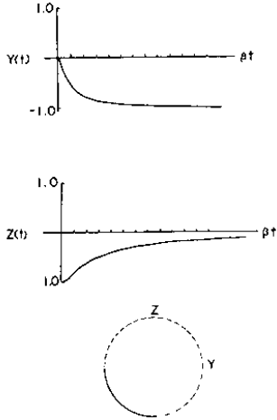
FIG. 4. Solutions of the secular equations for \alpha = \gamma = 0 and \lambda = 0.99\beta .
