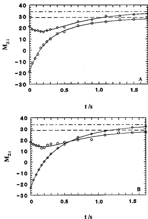
FIGURE 3 Time course of magnetization in SIT experiments for V9(a) of GCN4-IzK at 28.7°C. Solvent and peptide chain formality as in Fig. 1. Open circles : experimental F_a^{V9} magnetizations; open diamonds : experimental F_b^{V9} magnetizations. Solid curves : solutions to kinetic differential equations with parameters from Bayesian analysis. Dashed horizontal lines : calculated asymptotes for F_a^{V9} sites; dot-dashed horizontal lines : calculated asymptotes for F_b^{V9} sites. (A) F_a^{V9} inverted. (B) F_b^{V9} inverted.
