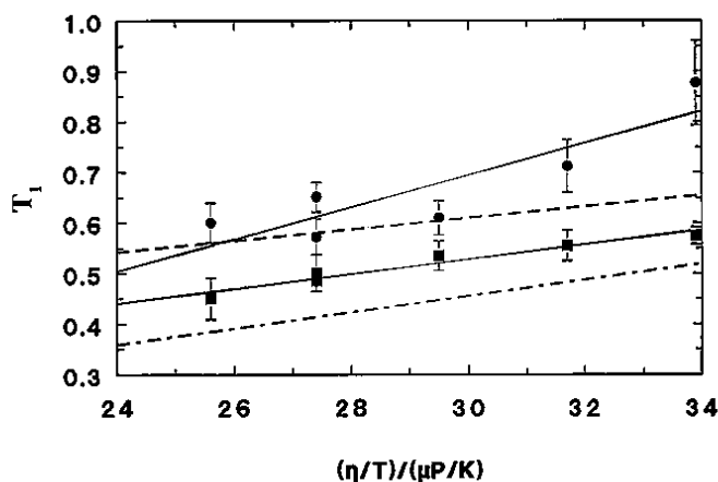
FIGURE 4 SIT-derived T_1 values at site V9(a) of GCN4-IzK versus \eta(T)/T . Filled squares : F_a^{V9} ; filled circles : F_b^{V9} . Error bars are from Bayesian probability distributions. Dot-dashed line : prior result for F_a^{L13} ; dashed line : prior result for F_b^{L13} .
