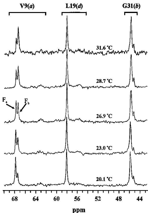
FIGURE 1 ^{13}\text{C}^{\alpha} -NMR spectra of GCN4-lzK in (\text{NaCl})_{100}(\text{NaPi})_{50} (\text{D}_2\text{O})_{5514}(7.4) near room temperature. Formal concentration of peptide chains, 1.24 mM. Regions for full range of resonances at the respective labeled sites V9(a), L19(d), and G31(b) are marked. V9(a) resonances assigned to local folded form favored at low T ( F_a^{V9} ) and at moderate T ( F_b^{V9} ) are also marked.
